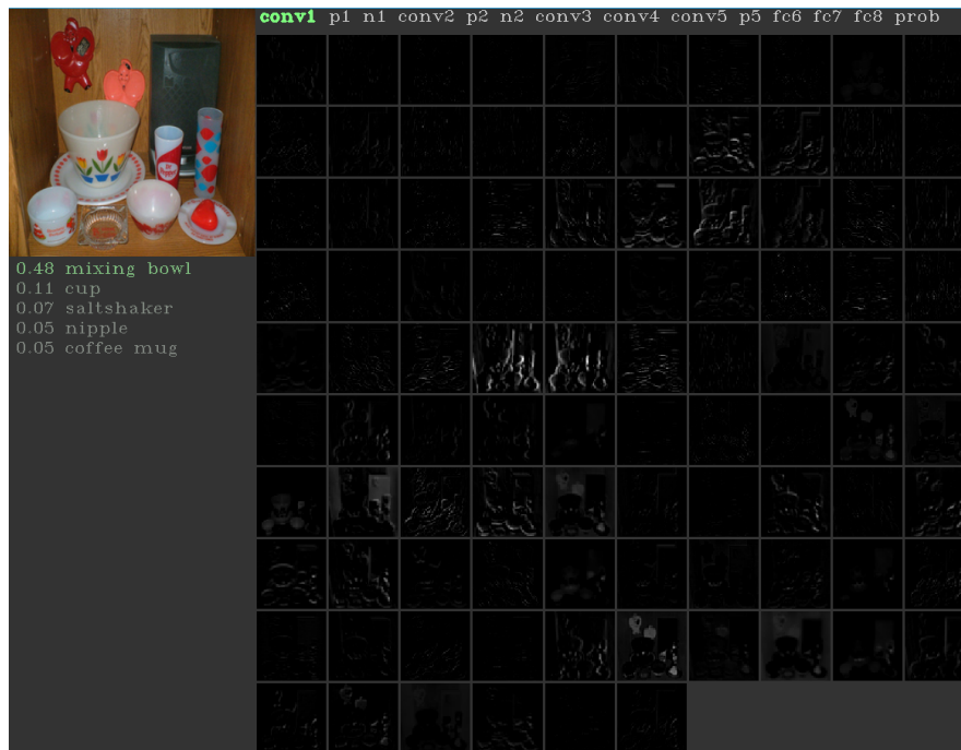
Fig. 2 Pixel based display. Activations of first convolutional layer generated with the DeepVis toolbox from [80] from https://github.com/yosinski/deep-visualization-toolbox/ .
