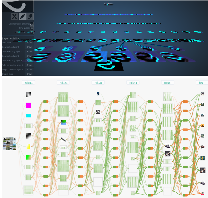
Fig. 5 Node-link diagrams of DNNs. Top: Example from [26] taken with the online application at http://scs.ryerson.ca/~aharley/vis/conv/ . Bottom: screenshot of the CNNVis system [44] taken with the online application at http://shixialiu.com/publications/cnnvis/demo/ .
